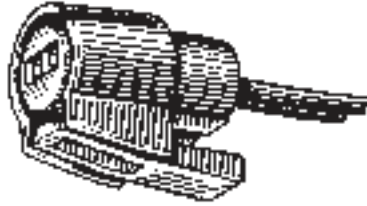
16513 (GM: 12085521) Replacement harness connector used on GM V-5 Air Conditioning Switches. Fits GM High Pressure Switch 6551917 and others. Index slot is at the one o'clock position. Features two 9" long 18 gauge wire leads. UNIT PACKAGE: 1
