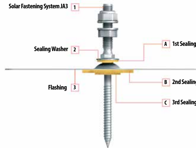
Sealing in three levels on THREE TAB Shingle Roofs
