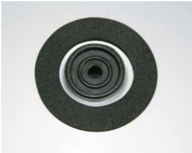
Bottom view – 2nd and 3rd sealing underneath Flashing
