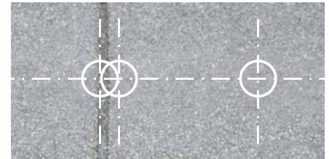
Individual positioning of the fastener - close to, or even right on a low between two highs - without shimming
